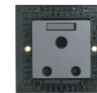
15A 200-250V 1 Gang Socket with Shutter & Earth
